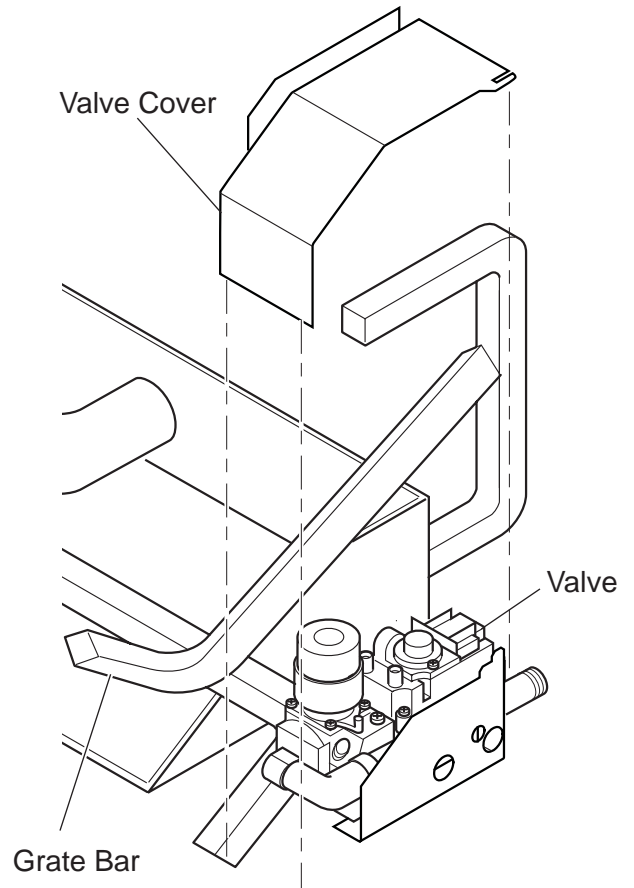
Figure 6 - Placing Cover on Milli-volt Control
